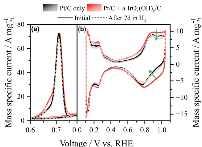
Figure 8. CO-stripping voltammograms (a) 1st and 2nd, (b) 3rd cycle of CV performed prior to cell reversal test. Pt/C only reference (black) and carbon-supported amorphous iridium oxyhydroxide 30 wt.% a-IrO x (OH) y /C (red) containing sample, initially after break-in of the MEAs (solid line) and after seven days of continuous operation in H 2 (dashed line). Single cell setup, 20 mV s -1 scan rate, 35 °C cell temperature, RH of 100% for the supplied gases, ambient pressures and 50/500 nccm constant flow rates with N 2 /5% H 2 (balance sat. N 2 ) for the anode and cathode, respectively.
