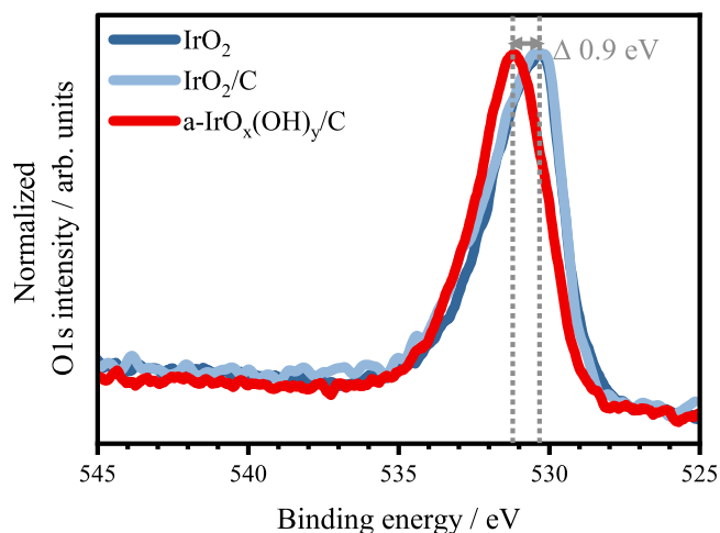
Figure 3. Normalized XPS O 1s core spectra of unsupported \text{IrO}_2 (dark blue line), carbon-supported crystalline iridium oxide 30 wt.% \text{IrO}_2/\text{C} (light blue line), and carbon-supported amorphous iridium oxyhydroxide 30 wt.% \text{a-IrO}_x(\text{OH})_y/\text{C} (red line). The arrows indicate the shift in binding energy of the peak maxima between the measured samples.
