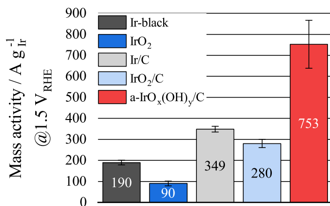
Figure 4. Mass activities towards the oxygen evolution reaction (OER) derived from RDE measurements ( 10 \text{ mV s}^{-1} , 1600 rpm, 60^\circ\text{C} , air sat. 0.5 \text{ M H}_2\text{SO}_4 ) for the following OER co-catalysts: unsupported Ir-black (black), and \text{IrO}_2 (dark blue), carbon-supported metallic iridium 30 wt.% Ir/C (grey), carbon-supported crystalline iridium oxide 30 wt.% \text{IrO}_2/\text{C} (light blue), carbon-supported amorphous iridium oxyhydroxide 30 wt.% \text{a-IrO}_x(\text{OH})_y/\text{C} (red). The error bars indicate the range between three individual measurements.
