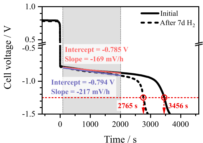
Figure 5. Representative cell voltage progression for membrane electrode assemblies (MEAs) containing Ir-black as oxygen evolution co-catalyst during cell reversal experiments, determined both initially after break-in of the MEAs (black solid line) and after seven days of continuous operation in \text{H}_2 (black dotted line). Grey area indicates the range for the linear fit. The intersection of the measured data with -1.25 \text{ V} (red dotted line) describes the cell reversal time. Single cell setup, 0.2 \text{ A cm}^{-2}_{\text{geo}} , 80^\circ \text{C} cell temperature, RH of 100% for the supplied gases, 150/150 \text{ kPa}_{\text{abs,inlet}} total pressures and 1000/5000 \text{ nccm} constant flow rates for the anode and cathode, respectively.
