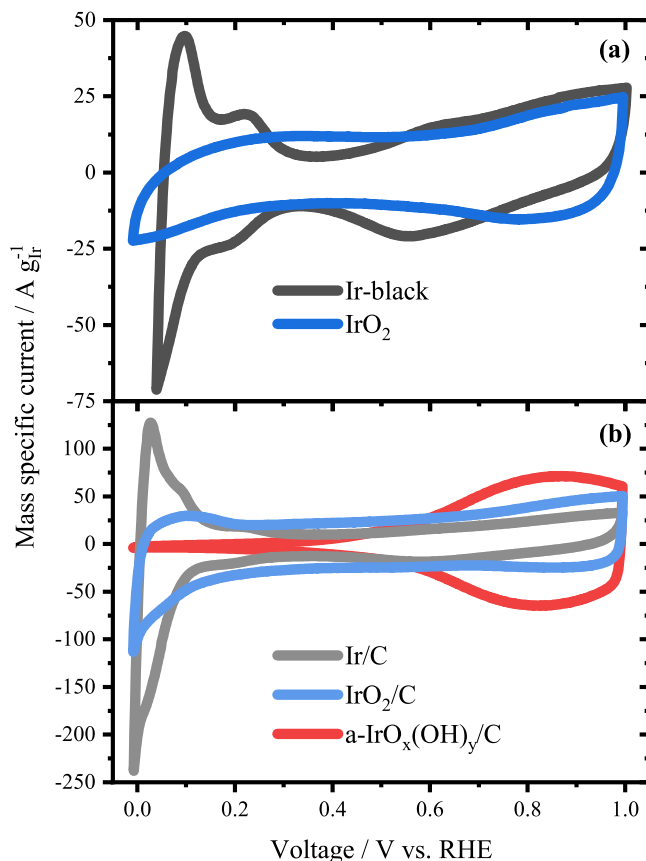
Figure 1. Cyclic voltammograms (CVs) of the oxygen evolution (OER) co-catalysts, (a) unsupported Ir-black (black line), and \text{IrO}_2 (dark blue line), (b) carbon-supported metallic iridium 30 wt.% Ir/C (grey line), carbon-supported crystalline iridium oxide 30 wt.% \text{IrO}_2/\text{C} (light blue line), and carbon-supported amorphous iridium oxyhydroxide 30 wt.% a- \text{IrO}_x(\text{OH})_y/\text{C} (red line). CVs: RDE, 100 \text{mV s}^{-1} , 60 °C, \text{N}_2 sat. 0.5 M \text{H}_2\text{SO}_4 .
