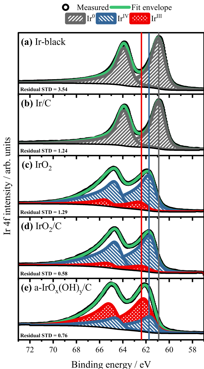
Figure 2. XPS Ir 4f with core spectra (black circles), fitted chemical states— \text{Ir}^0 (grey shaded region), \text{Ir}^{\text{III}} (red shaded region), \text{Ir}^{\text{IV}} (blue shaded region)—and the resulting fit envelope (green line) of (a) unsupported Ir-black, (b) carbon-supported metallic iridium 30 wt.% Ir/C, (c) \text{IrO}_2 , (d) carbon-supported crystalline iridium oxide 30 wt.% \text{IrO}_2/\text{C} , and (e) carbon-supported amorphous iridium oxyhydroxide 30 wt.% \text{a-IrO}_x(\text{OH})_y/\text{C} . Colored vertical lines represent the binding energy position of the main Ir 4f peaks of \text{Ir}^0 , \text{Ir}^{\text{III}} and \text{Ir}^{\text{IV}} .
