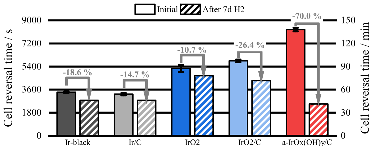
Figure 7. Bar chart showing the cell reversal time at -1.25 V for employed oxygen evolution co-catalysts determined both initially after break-in of the MEAs (solid bars) and after seven days of continuous operation in H_2 (striped bars). The error bars indicate the range between two individual measurements.
