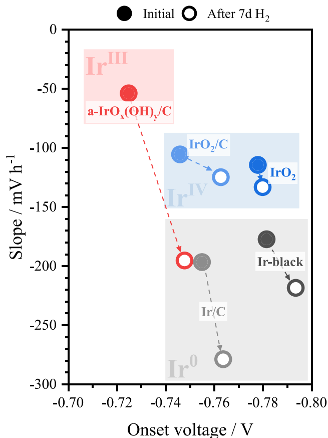
Figure 6. Employed oxygen evolution co-catalysts with the slope plotted over the onset voltage, derived from linear fit of cell voltage within the first 100–2000 s during cell reversal experiment (cf Fig. 5). Full circles: initially after break-in, open circles: after seven days of continuous operation in \text{H}_2 . The shaded rectangular clusters indicate the presumed predominant chemical state of the Ir co-catalysts, i.e. \text{Ir}^0 , \text{Ir}^{\text{III}} and \text{Ir}^{\text{IV}} .
